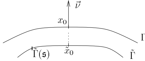
FIGURE 7. The curve \tilde{\Gamma} which supports \Delta\psi .
