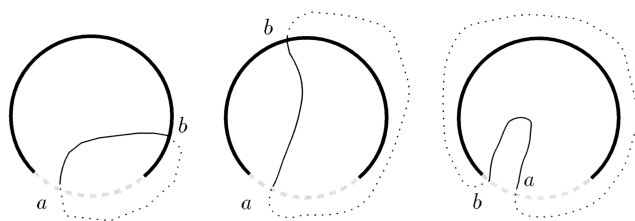
FIGURE 4. Describing \Sigma_i^j (or nearly it).
