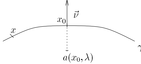
FIGURE 6. The position of the particle approaching x_0 .
