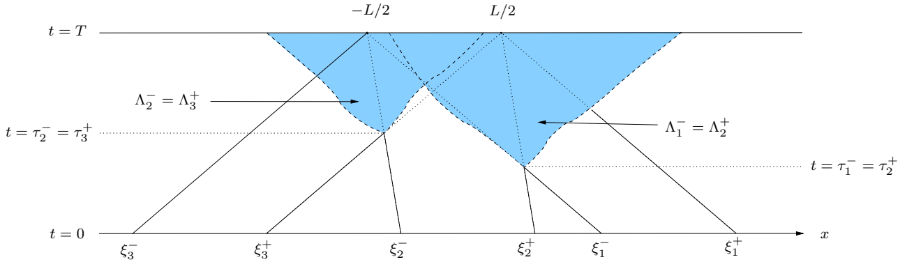
Figure 1: The sets \Lambda_i^\pm
