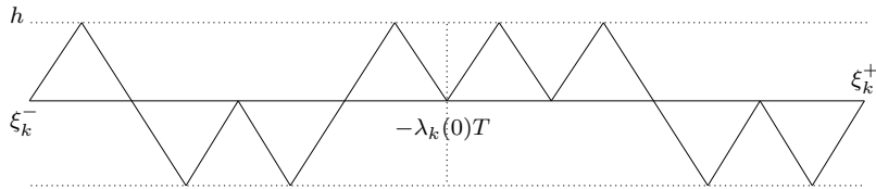
Figure 2: The function \beta_k^\iota for n = 8 and \iota = (0, 1, 1, 0, 0, 0, 1, 1) .
